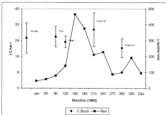
Figure 1. Oscillation of soil carbon stock (t C.ha -1 ) under pasture in relation to the seasonal cycle of rainfall in the Apiaú Colonization Area, Roraima, Brazil (Forest measured together Post 210).
