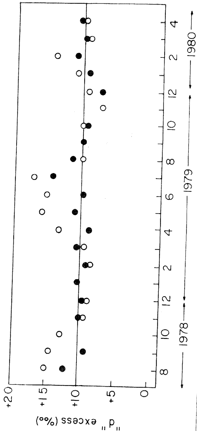
Fig. 6 - "d" - parameter of rain samples from Belém (o) and Manaus (●) on a monthly averaged basis.
