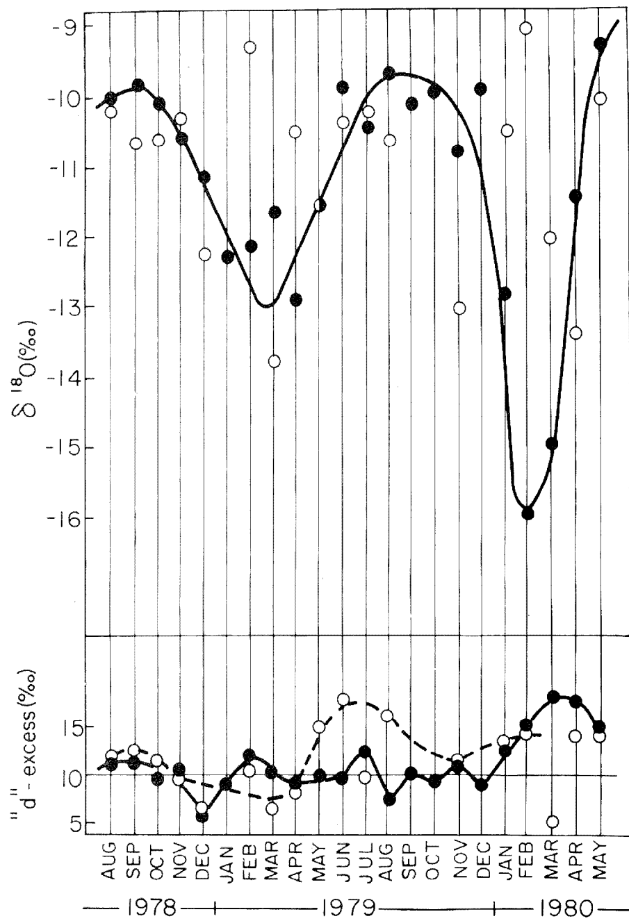
Fig. 8 – Monthly averaged isotopic values of daily vapour samples at Belém and Manaus ( \delta^{18}\text{O} values in upper curves, "d" - parameter at bottom of the figure). Belém data - \circ ; Manaus data - \bullet .
