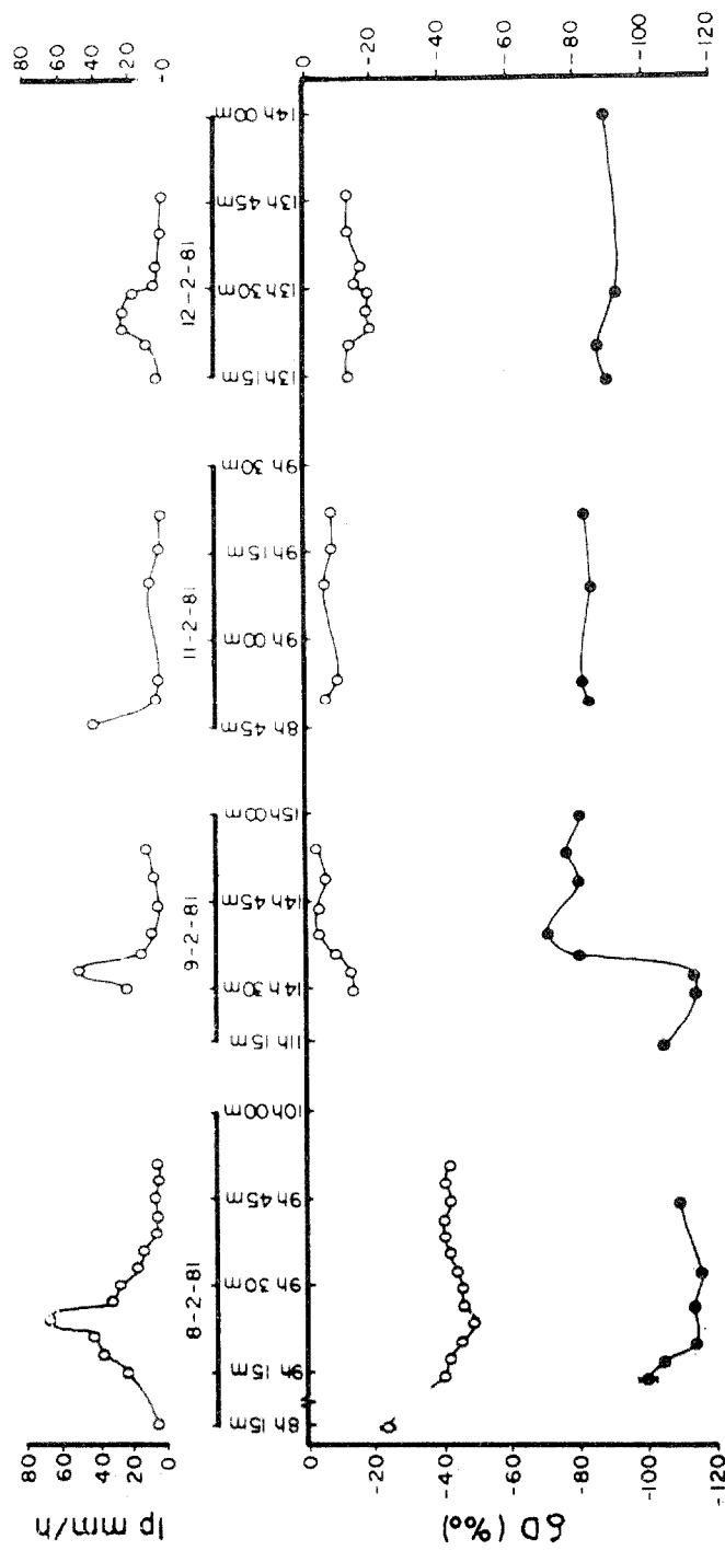
Fig. 9 — Isotope composition of simultaneously collected vapour and rain samples during showers at Manaus (10 minutes sampling intervals).
